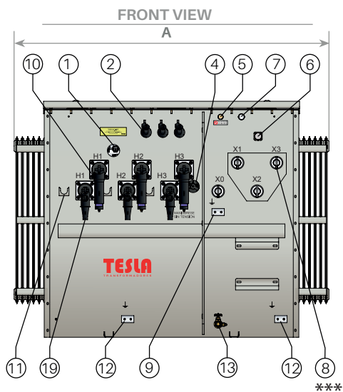
FRONT VIEW WITH ENCLOSURE
